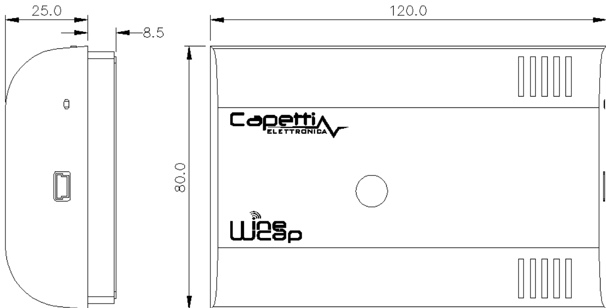
Picture 7 - Mechanical dimensions
