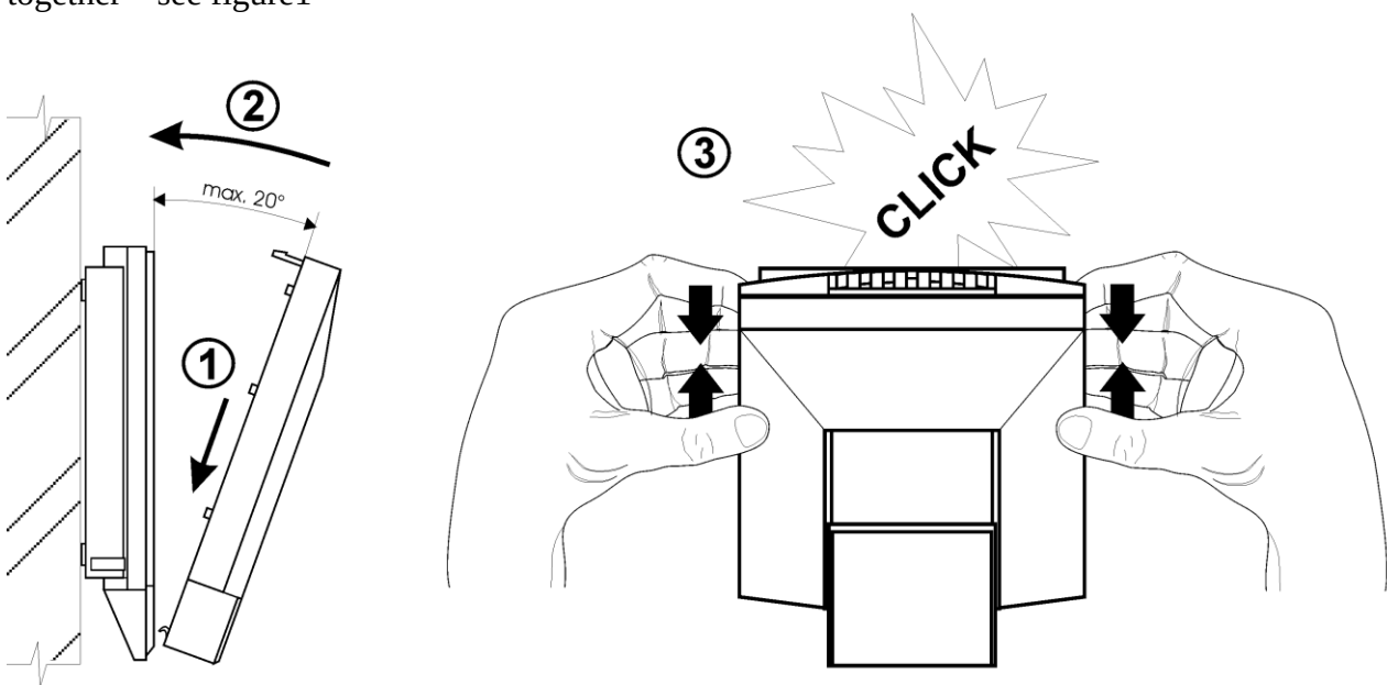
Figure1: Device mounting
