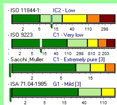
Corrosivity classification
