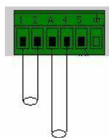
Differential Inputs
